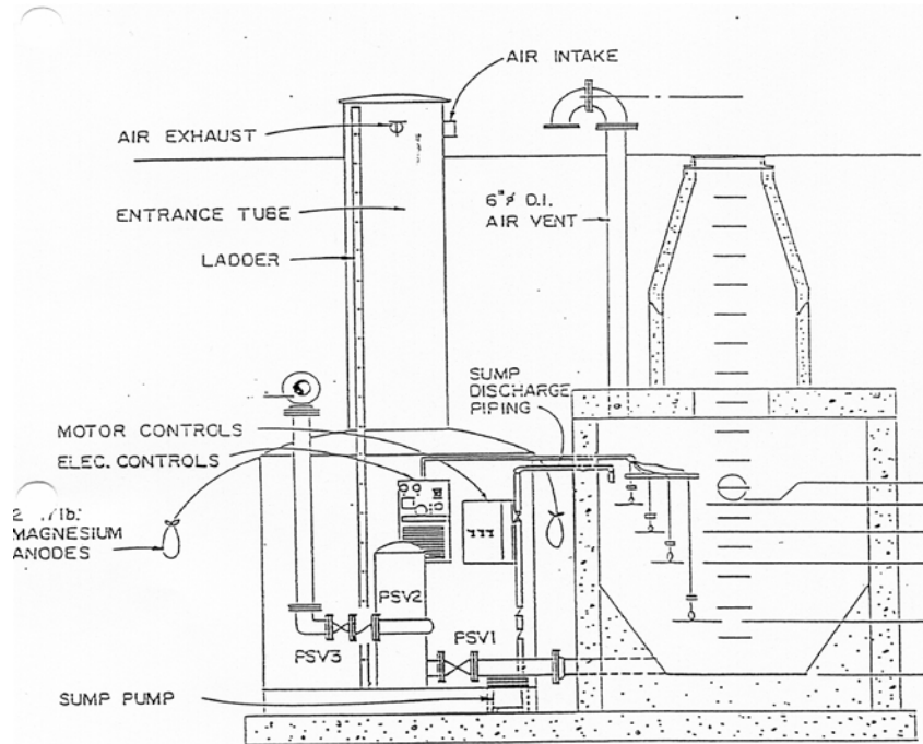
Package Wet Well/Dry Well Pump Station
