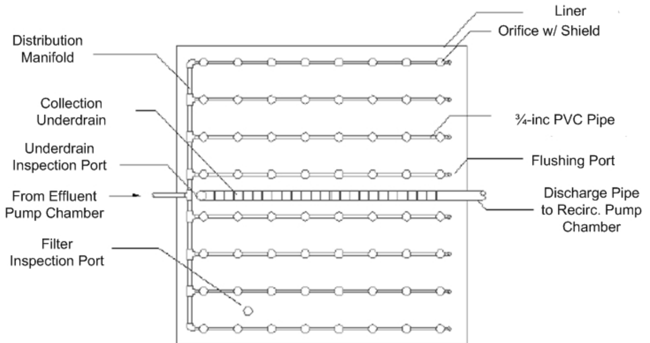
Recirculating Sand Filter Plan View
