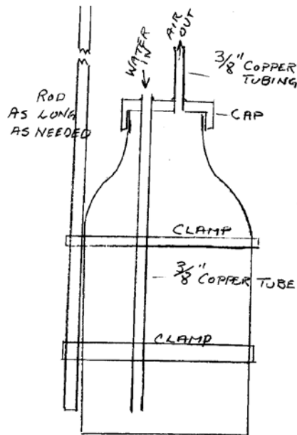
Sampling Device for Dissolved Oxygen Samples
